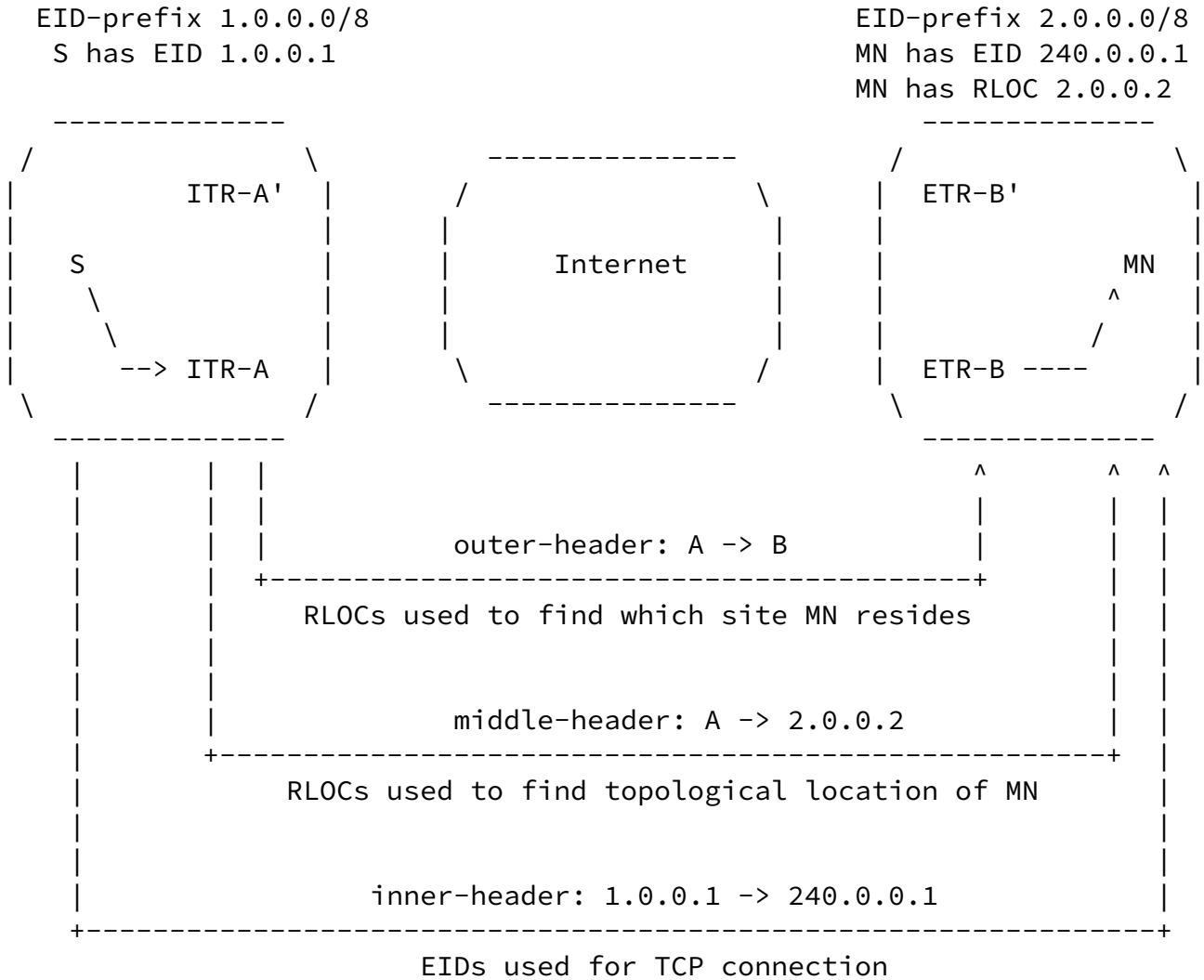
Figure 2: Mobile Node Roaming into a LISP Site
