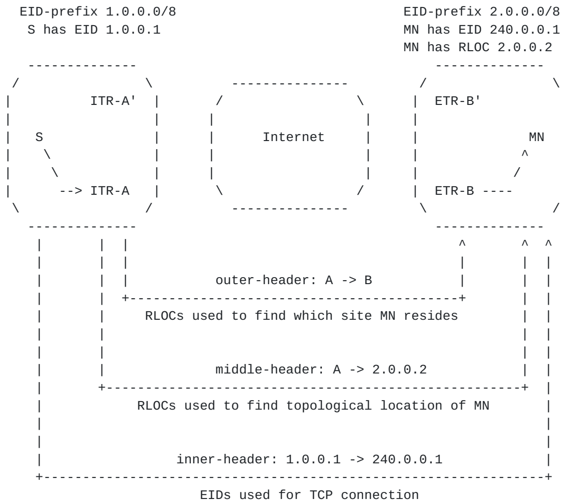
Figure 2: Mobile Node Roaming into a LISP Site
