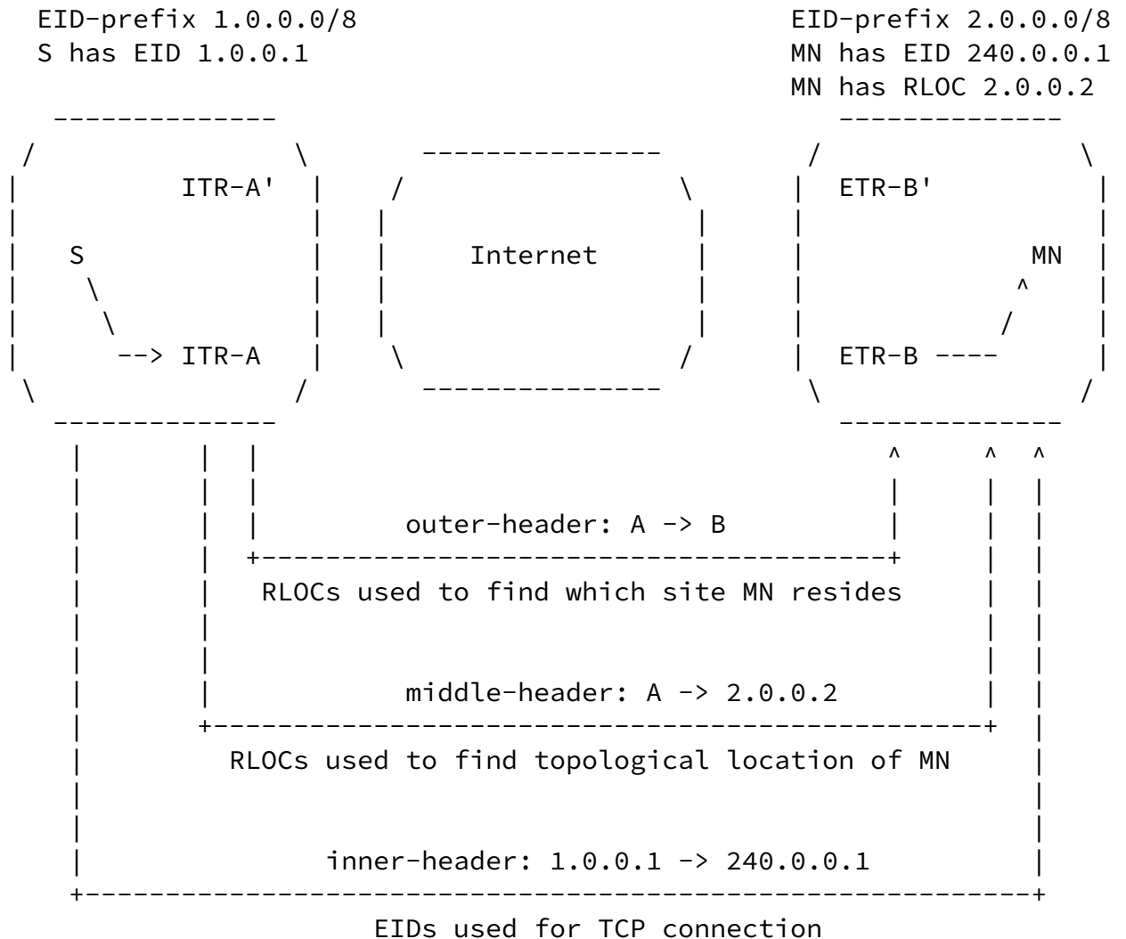
Figure 2: Mobile Node Roaming into a LISP Site
