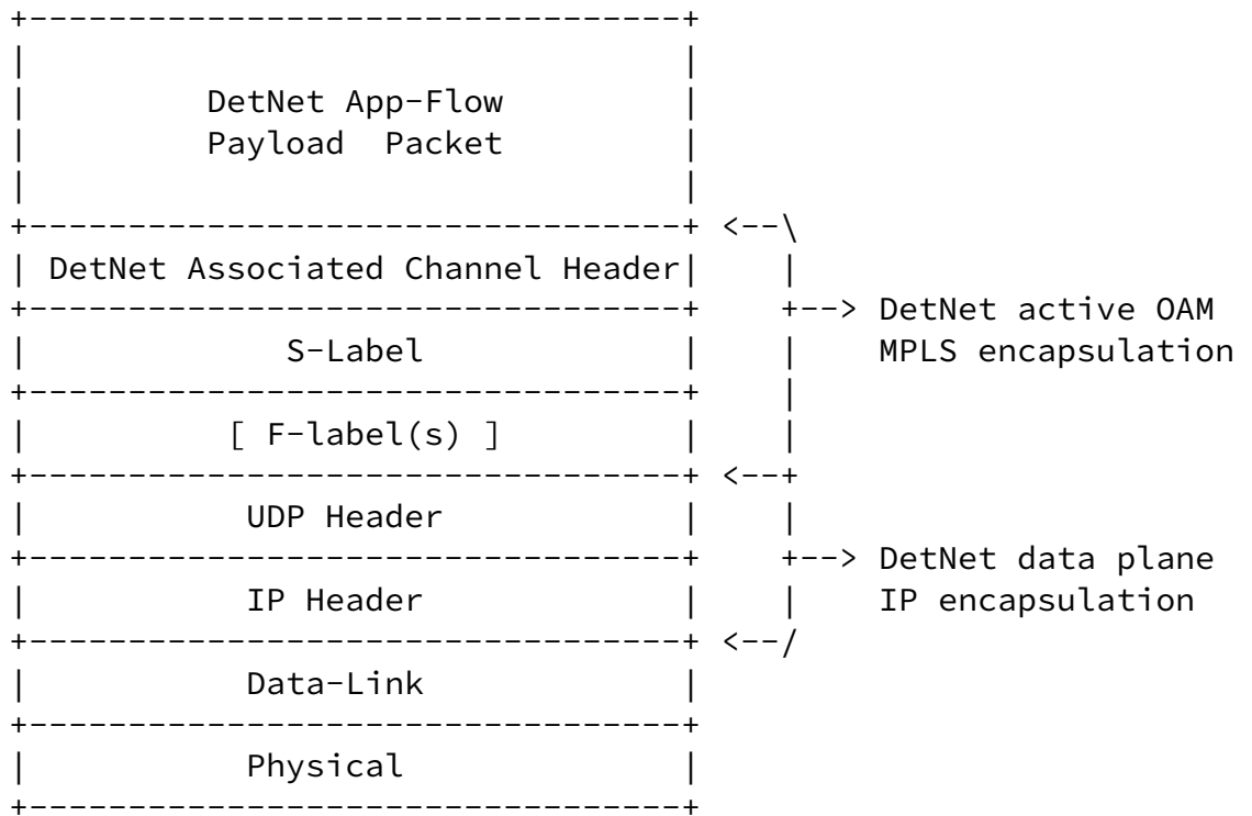
Figure 4: DetNet Active OAM Packet Encapsulation in MPLS-over-UDP/IP
