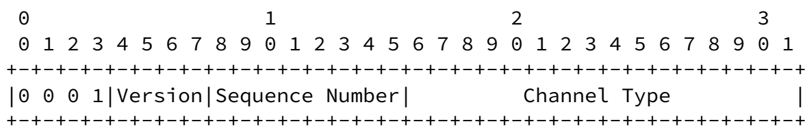
Figure 5: DetNet Associated Channel Header Format
