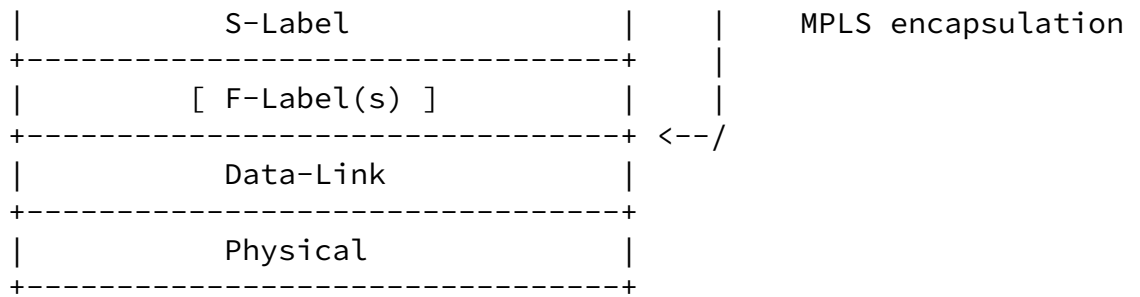
Figure 3: DetNet Active OAM Packet Encapsulation in MPLS Data Plane
