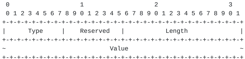
Figure 4: Telemetry Data TLV Format
