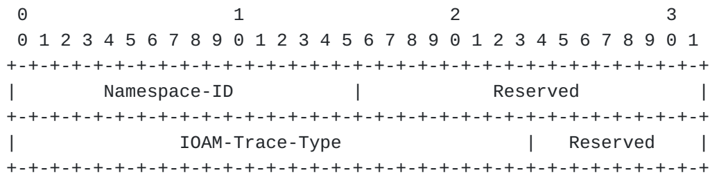
Figure 1: Hybrid Two-Step Trace IOAM Header
