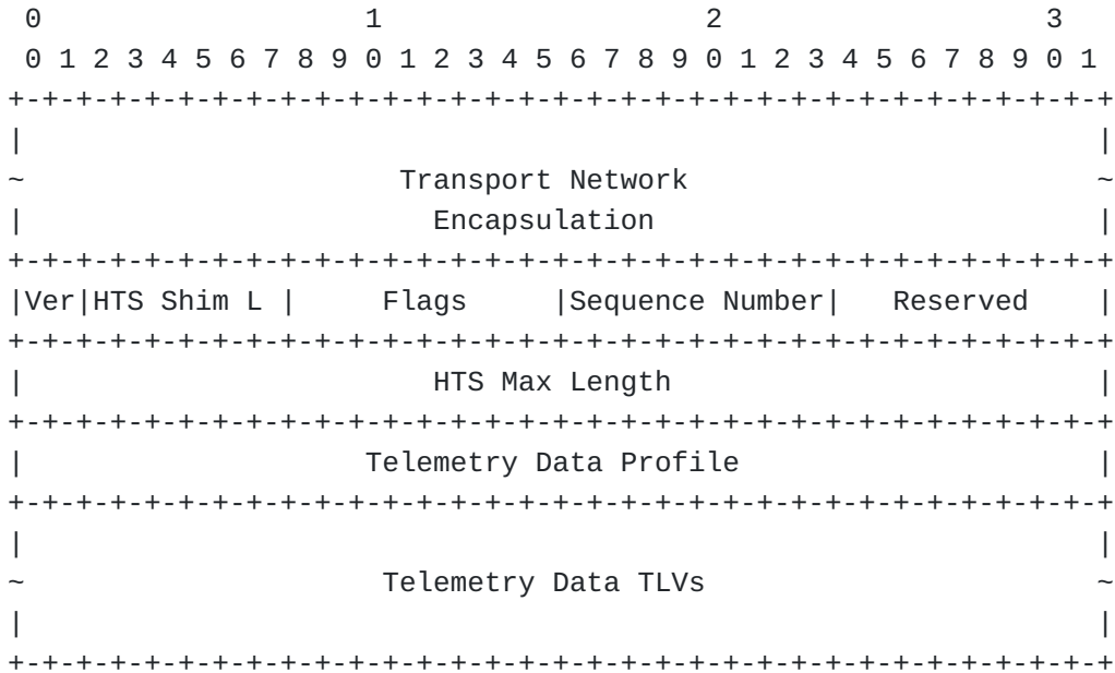
Figure 2: Follow-up Packet Format
