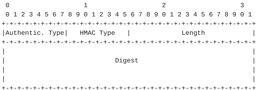
Figure 5: HMAC sub-TLV
