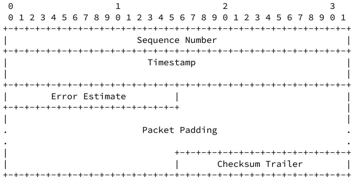
Figure 3 Checksum Trailer in OWAMP Test Packets
