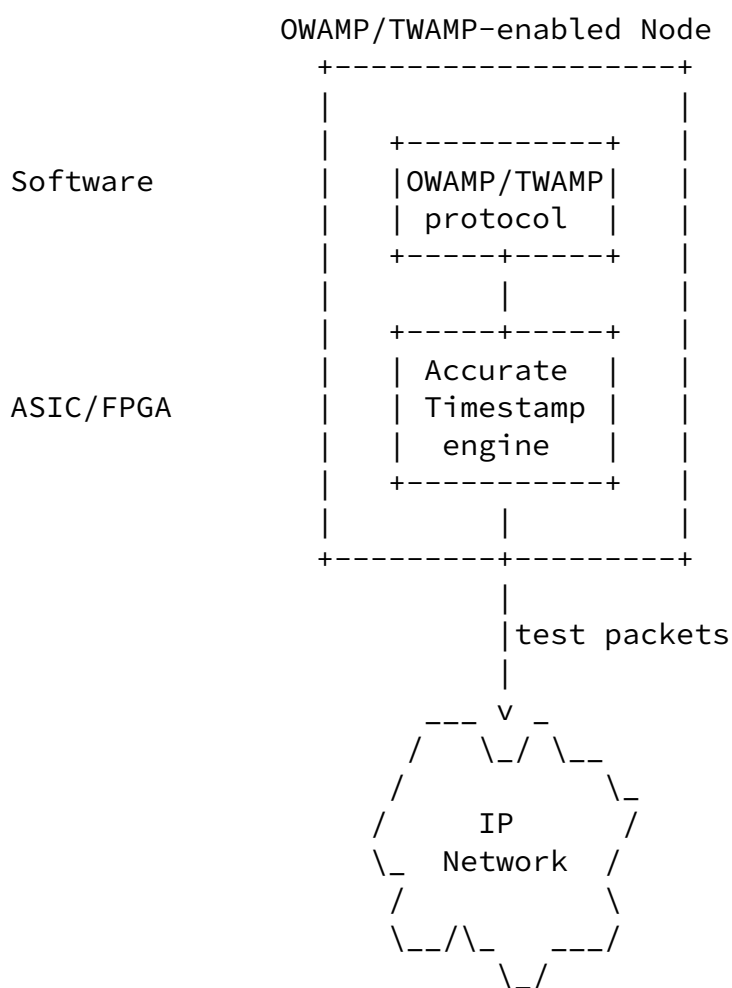
Figure 1 Accurate Timestamping in OWAMP/TWAMP
