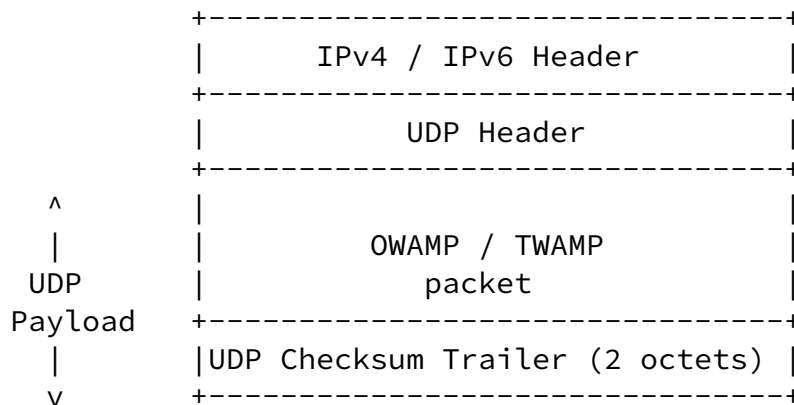
Figure 2 Checksum Trailer in OWAMP/TWAMP Test Packet
