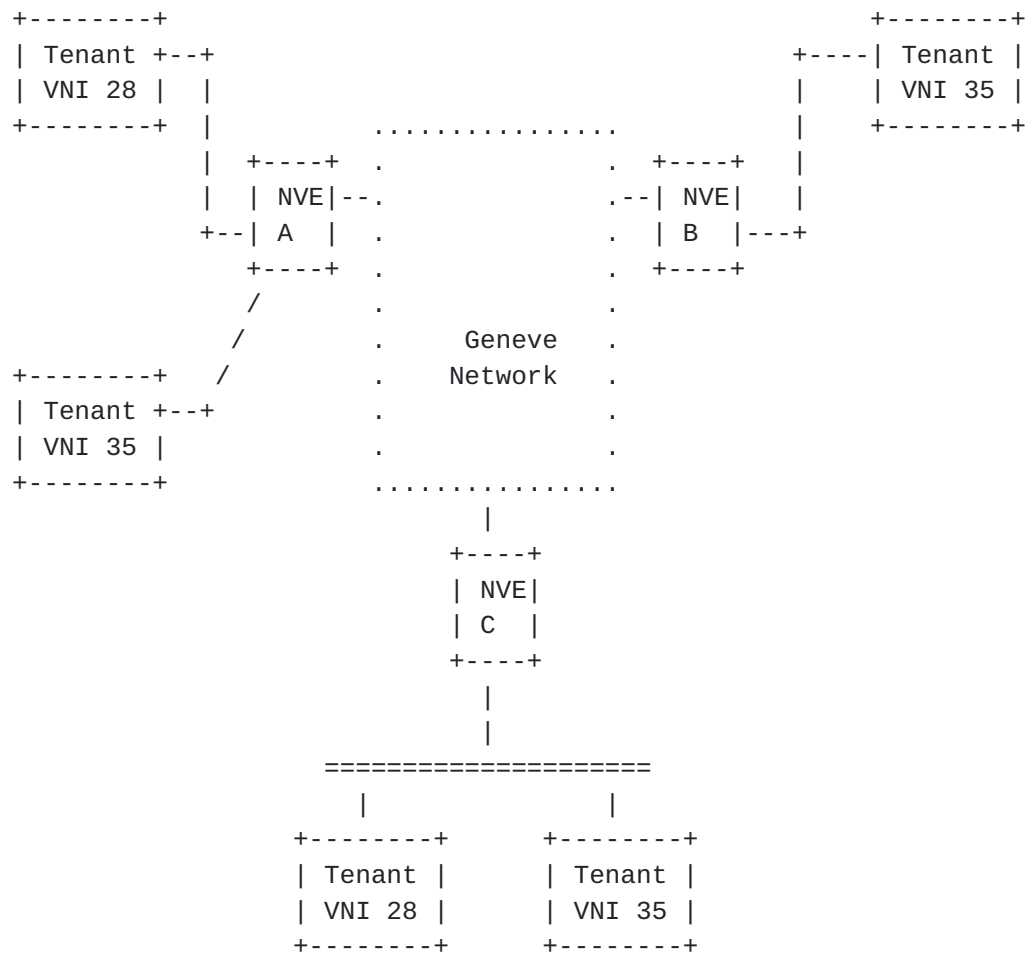
Figure 1: An example of a Geneve domain
