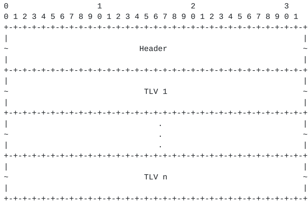
Figure 1: Basic message format
