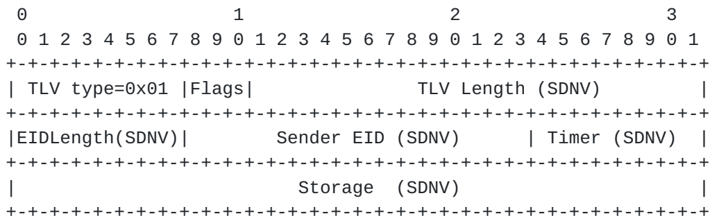
Figure 4: Hello TLV Format
