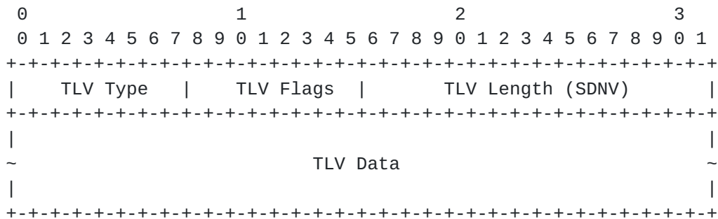
Figure 3: TLV Format
