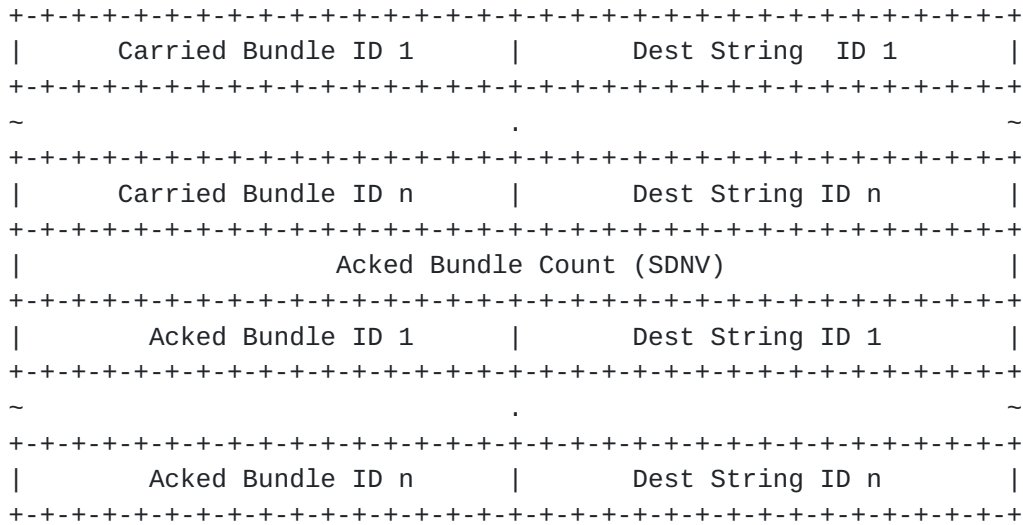
Figure 7: Social message TLV Format
