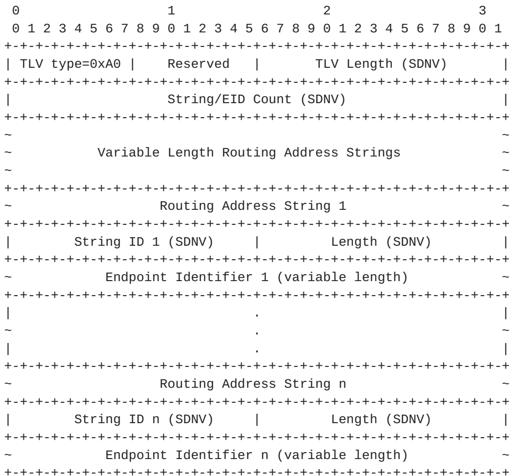
Figure 6: EID Dictionary TLV Format
