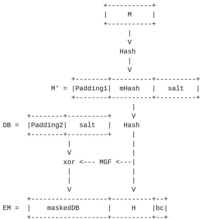
Figure 2: EMSA-PSS encoding operation. Verification operation follows reverse steps to recover salt, then forward steps to recompute and compare H.
