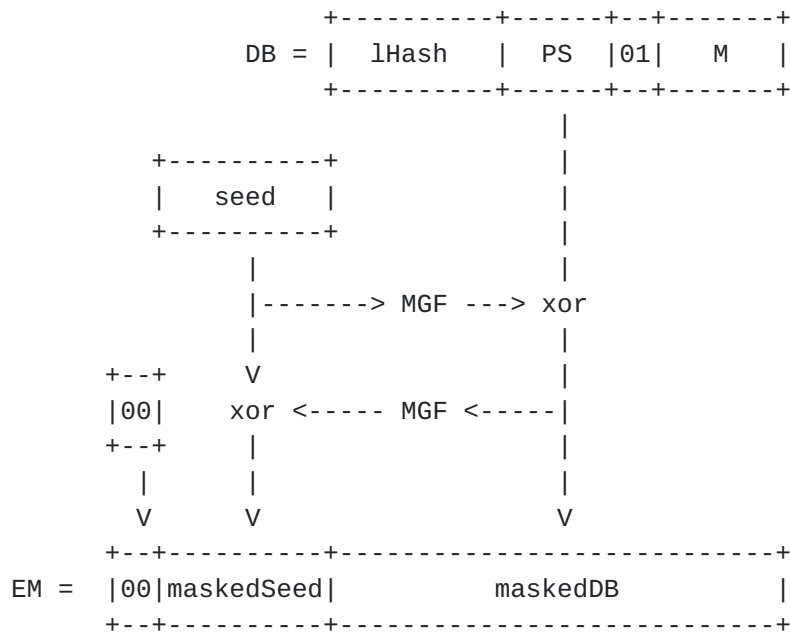
Figure 1: EME-OAEP encoding operation. lHash is the hash of the optional label L. Decoding operation follows reverse steps to recover M and verify lHash and PS.
