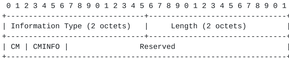
Figure 1: Compression Information TLV
