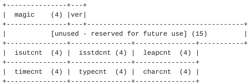
Figure 2: TZif Header
