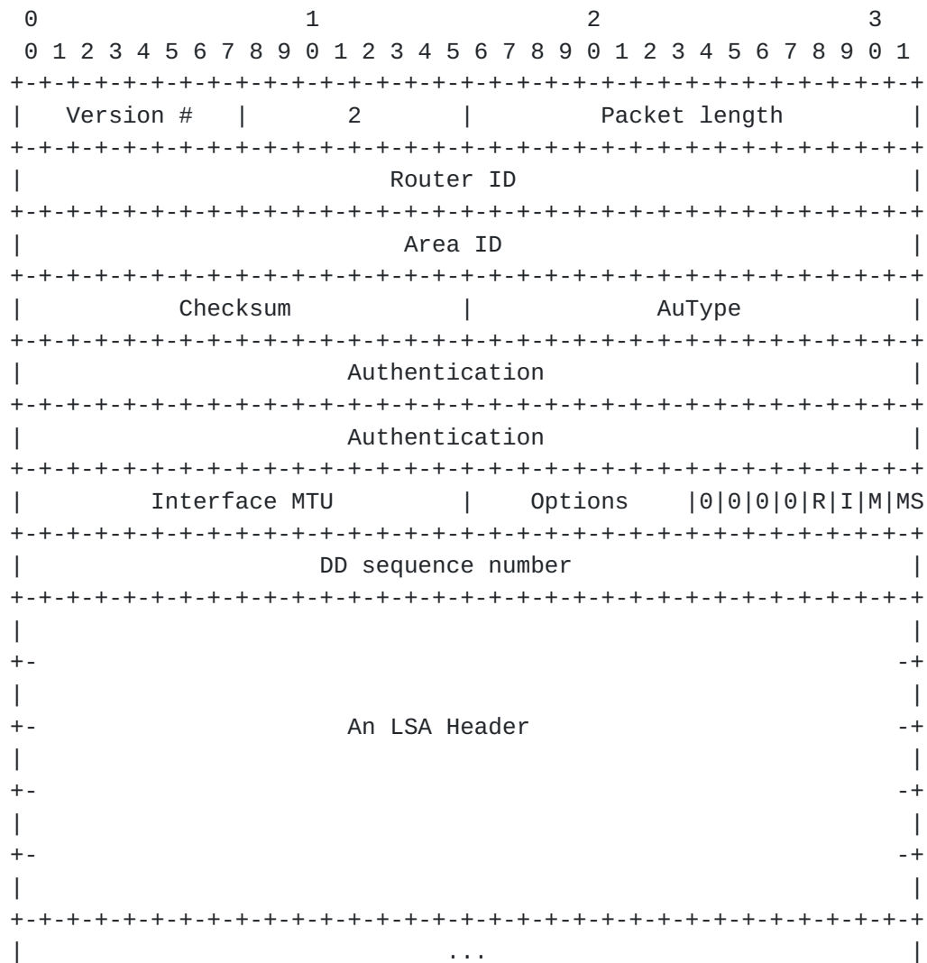
Figure 2. Modified DBD packet
