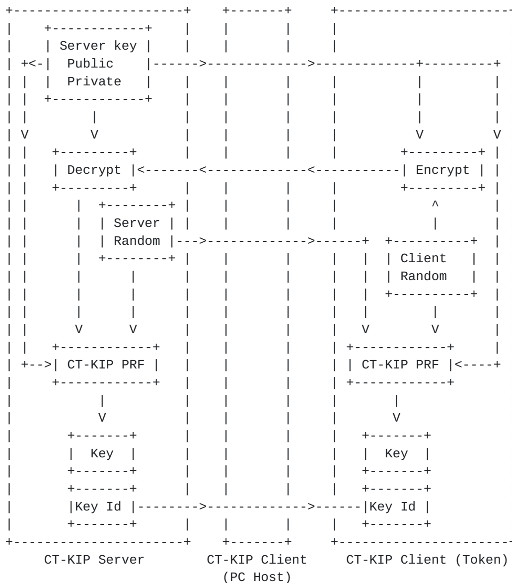
Figure 2: Principal data flow for CT-KIP key generation - using public server key
