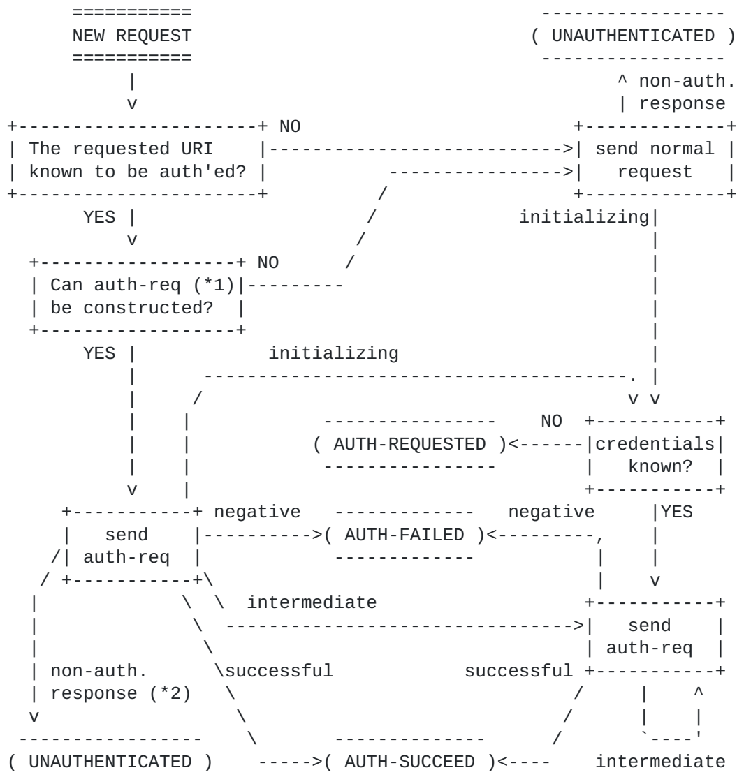
Figure 1: Generic state diagram for HTTP authentication
