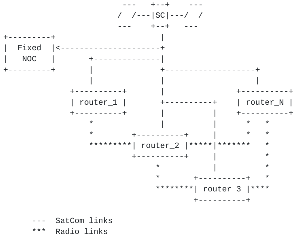
Figure 2: Monitoring with one-hop SatCom Reachback network
