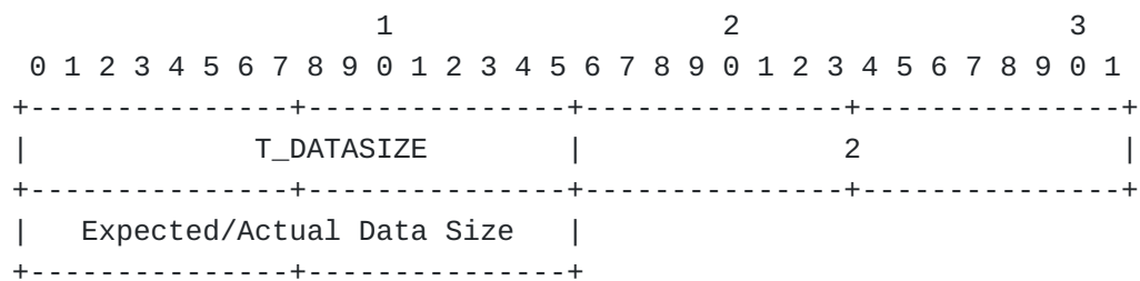
Figure 1: Expected/Actual Data size using RFC8609 encoding
