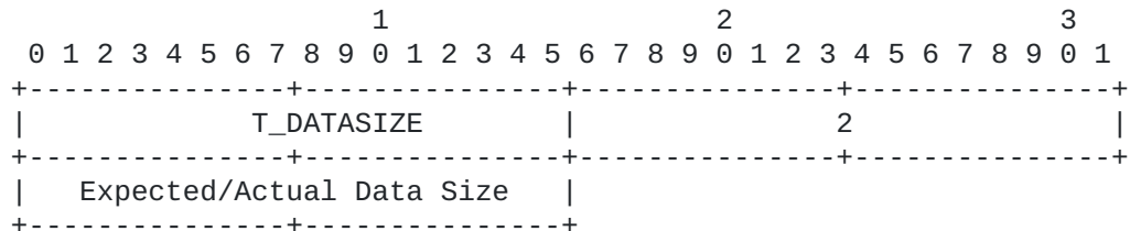
Figure 1: Expected/Actual Dataize using RFC8609 encoding
