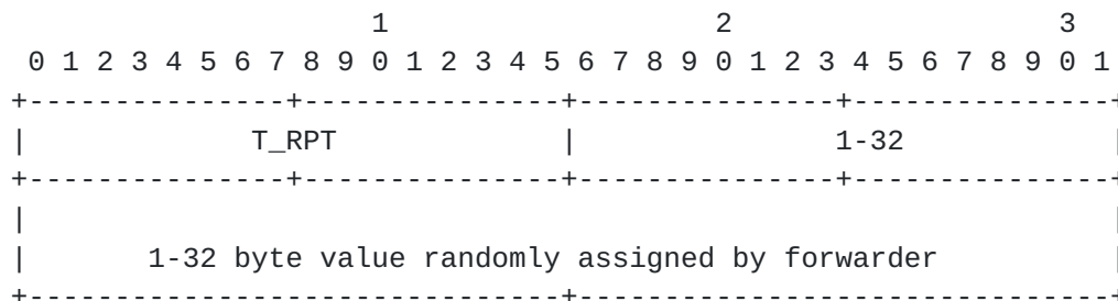
Figure 7: Reverse PIT-Token hop-by-hop TLV
