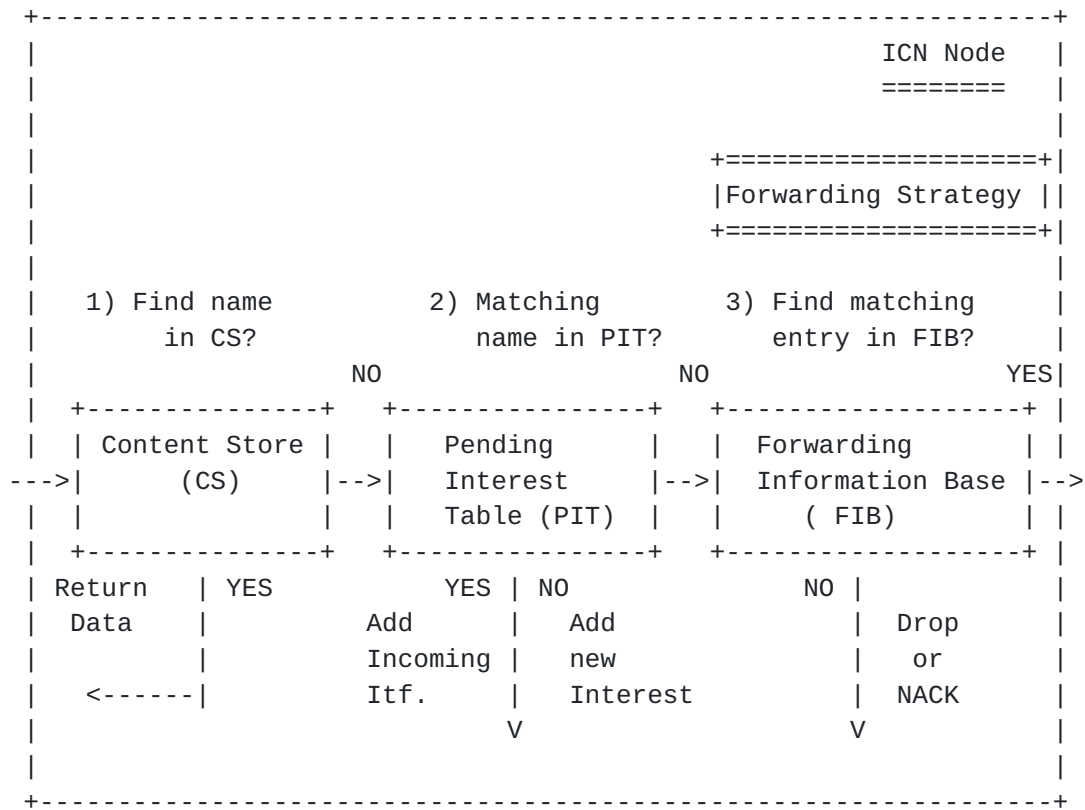
Figure 1: ICN forwarder structure
