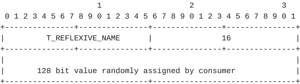
Figure 5: Reflexive Name segment type
