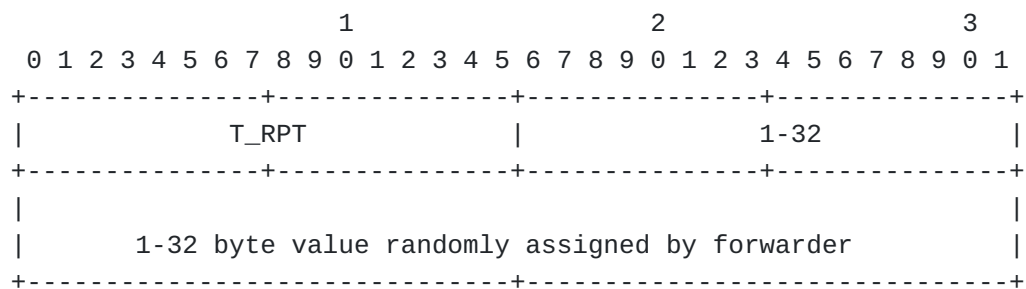
Figure 7: Reverse PIT-Token hop-by-hop TLV
