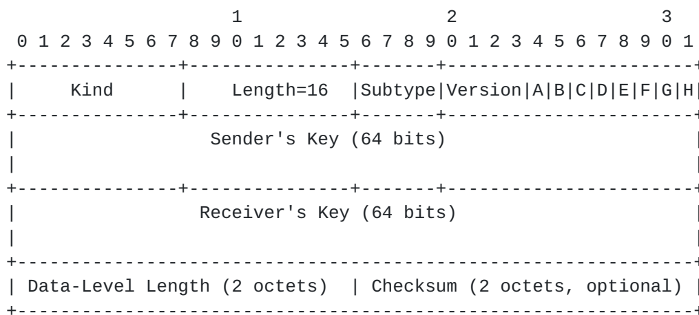
Format of the new MP_CAPABLE_EXT option.
