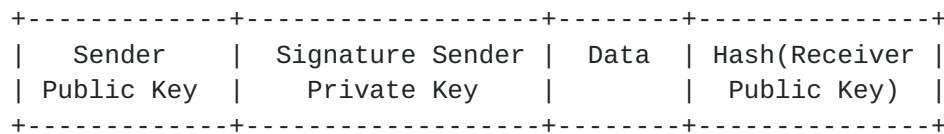
Figure 2.- Common transaction structure in a blockchain
