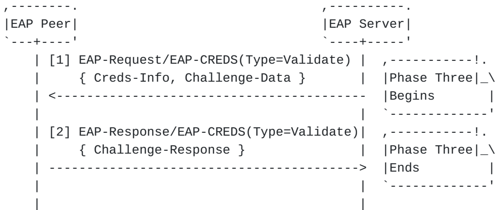
EAP-CREDS Phase Three Message Flow
