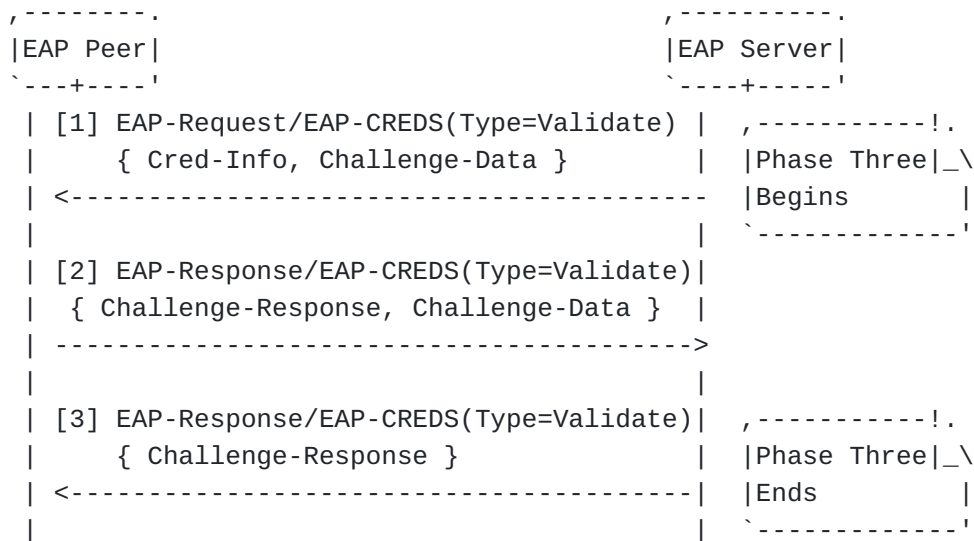
EAP-CREDS Phase Three Message Flow (Server-side Validation)
