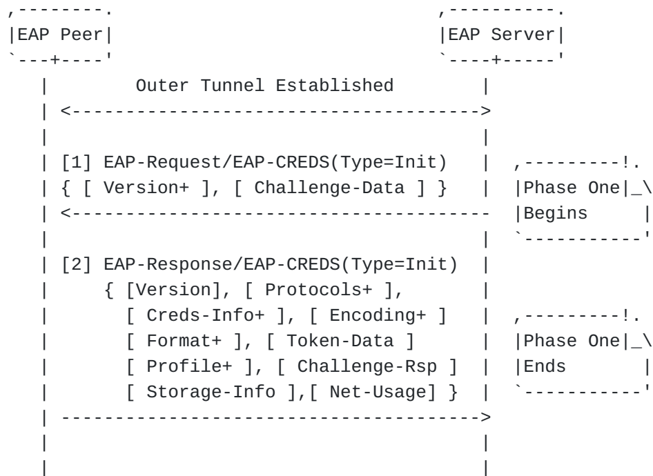
EAP-CREDS Phase One Message Flow
