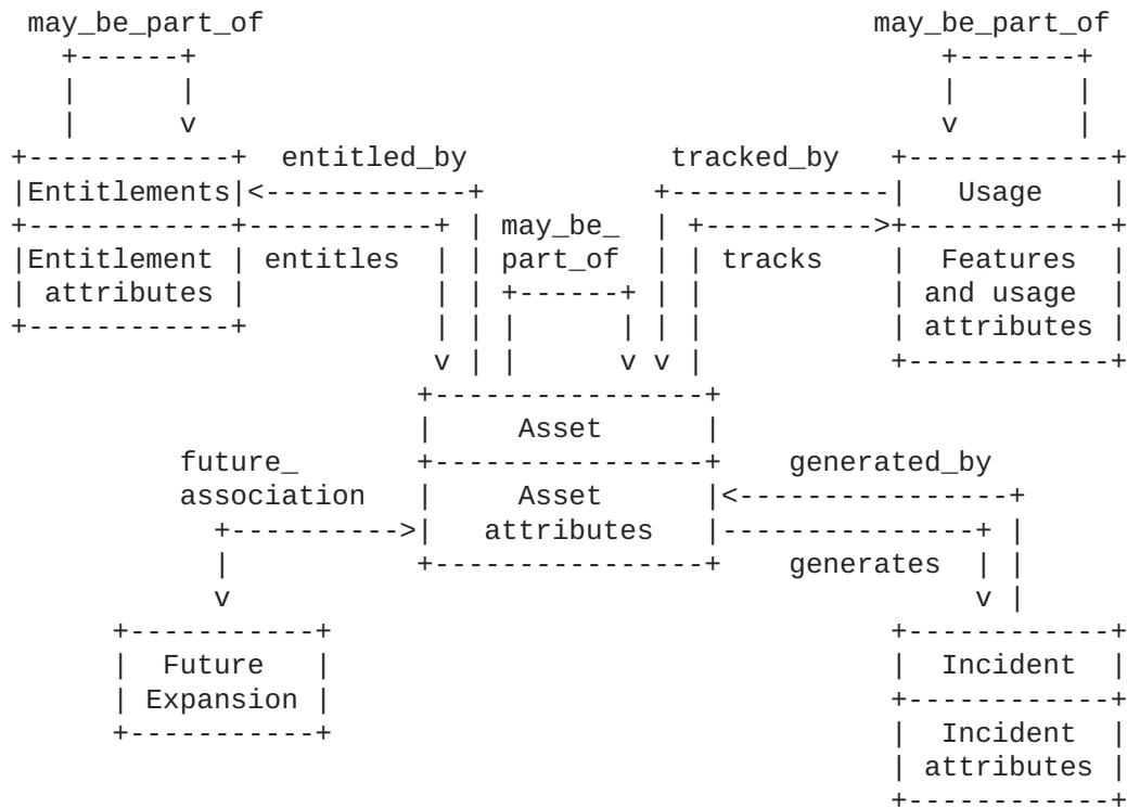
Figure 1: Information Model
