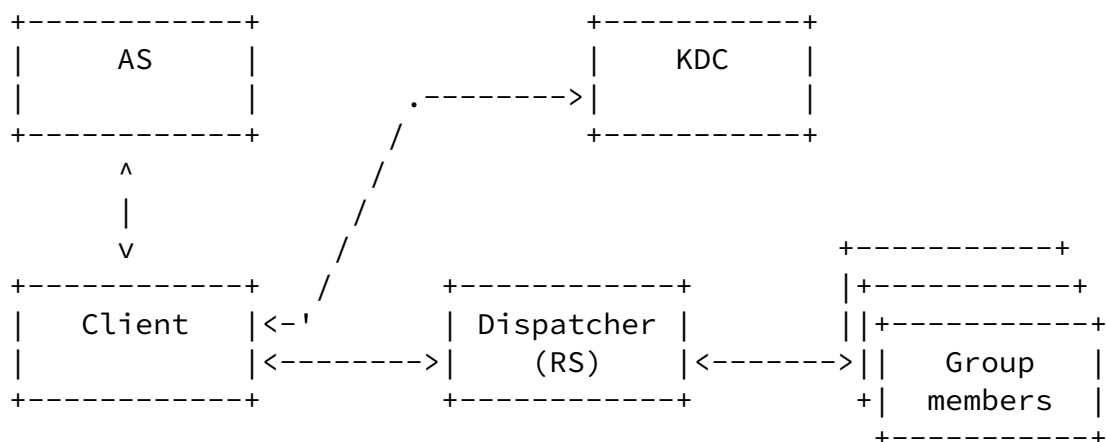
Figure 1: Key Distribution Participants
