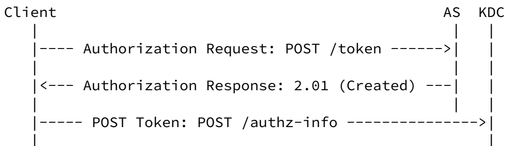
Figure 3: Message Flow of Join Authorization
