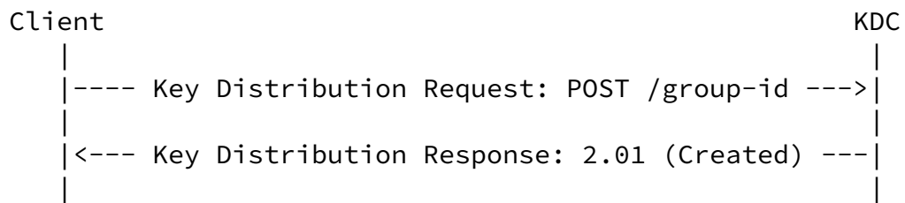
Figure 4: Message Flow of Key Distribution to a New Group Member
