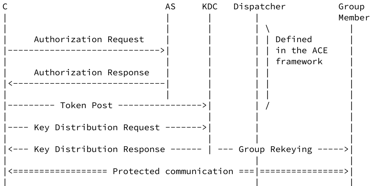
Figure 2: Message Flow Upon New Node's Joining
