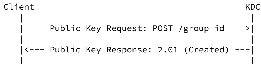
Figure 6: Message Flow of Public Key Request-Response
