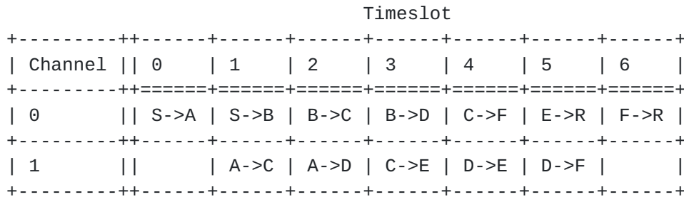
Figure 2: Packet Replication: S transmits twice the same data packet, to its DP (A) and to its AP (B).
