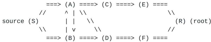
Figure 4: Unicast to DP with Overhearing: by employing Promiscuous Overhearing, DP, AP and the sibling nodes have more opportunities to receive the same data packet.
