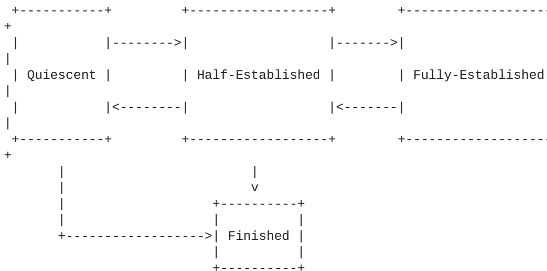
Figure 1: Multicast QUIC session states
