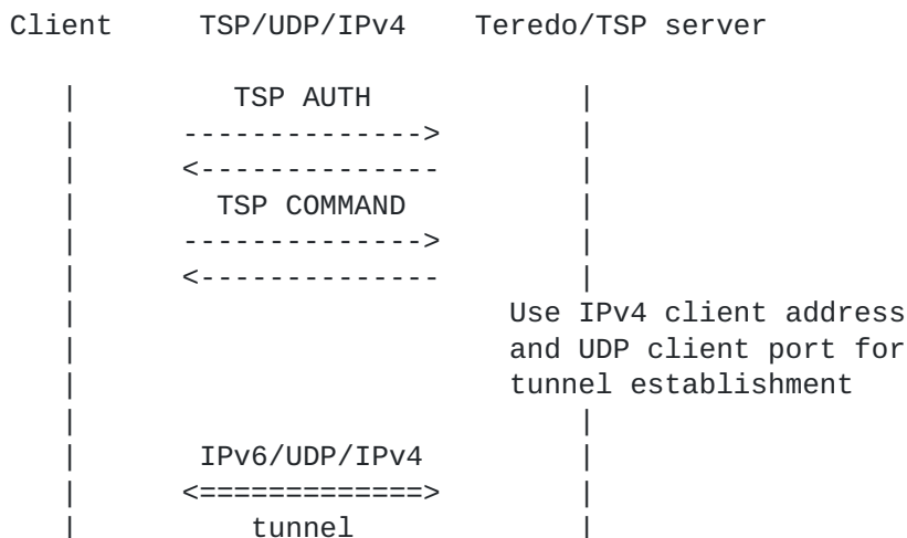
Figure 1: Client to server initial negotiation
