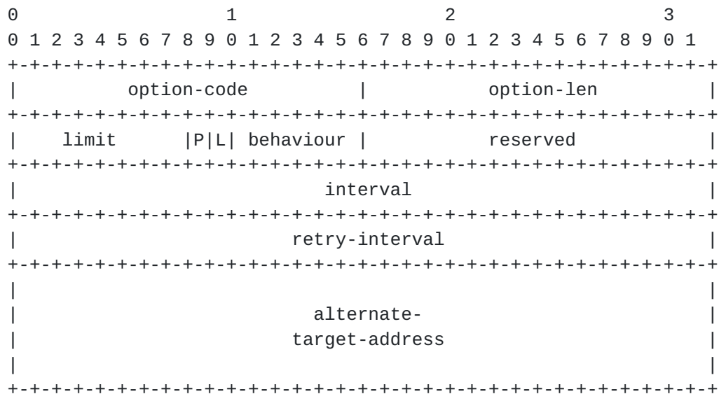
Figure 1: DHCPv6 IPoE Check Option Format
