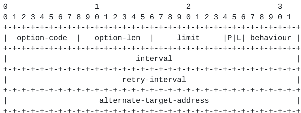
Figure 2: DHCPv4 IPoE Health Check Option Format
