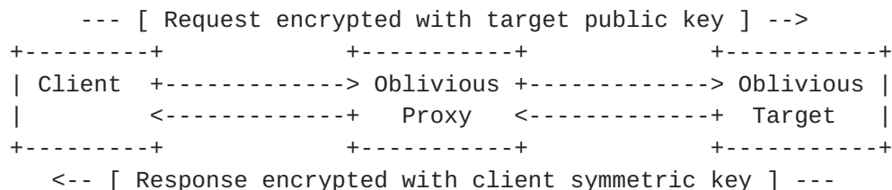
Figure 1: Oblivious DoH Exchange
