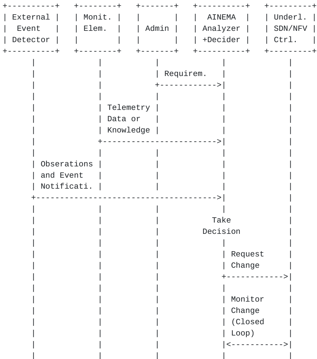
Figure 1: AINEMA Workflow
