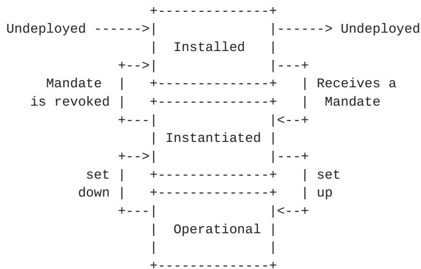
Figure 3: Life cycle of an Autonomic Function Agent
