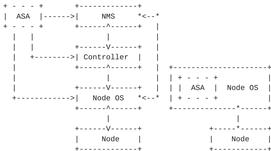
Figure 2: Interaction possibilities between ASA and Resources
