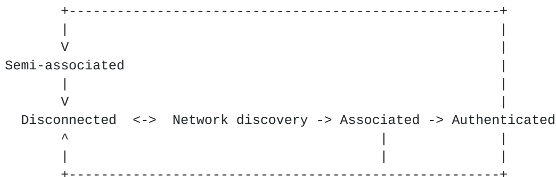
Node-F connectivity state machine.
