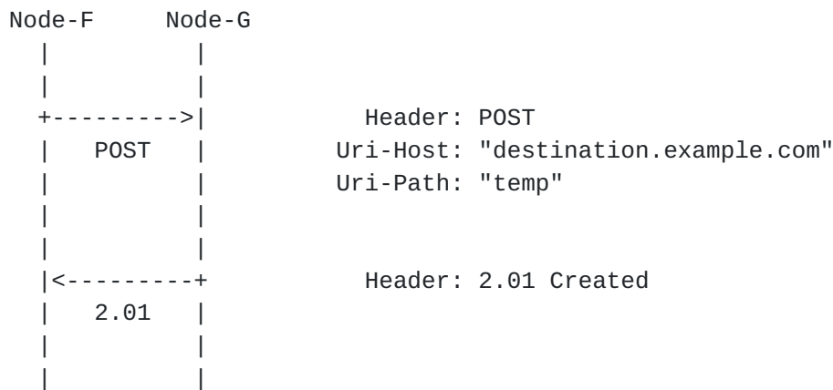
Sending a message in a semi-associated state.
