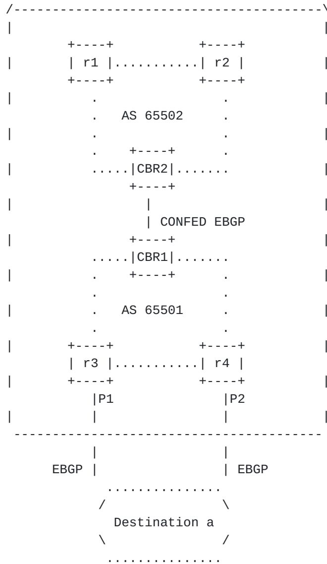
Figure 3: Confederation topology
