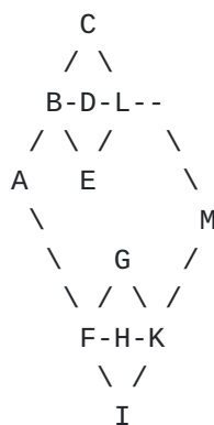
Figure 3: ECMP Topology Example
