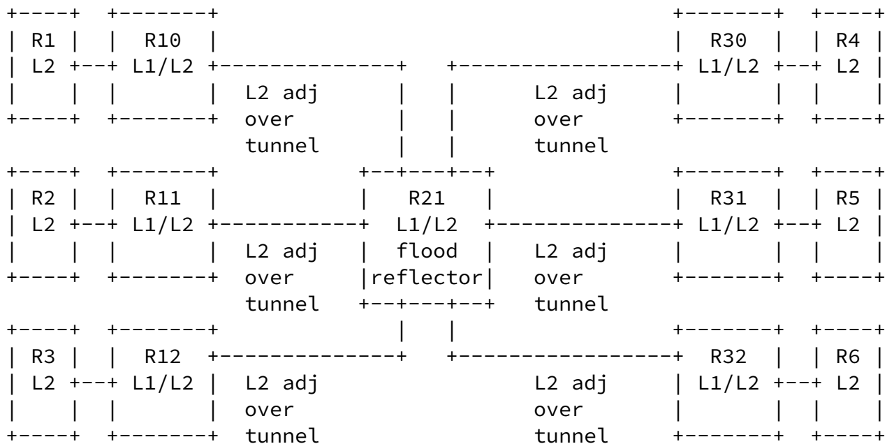
Figure 3: Example topology represented in L2 with L2 adjacencies from each L1/L2 node to a single flood reflector
