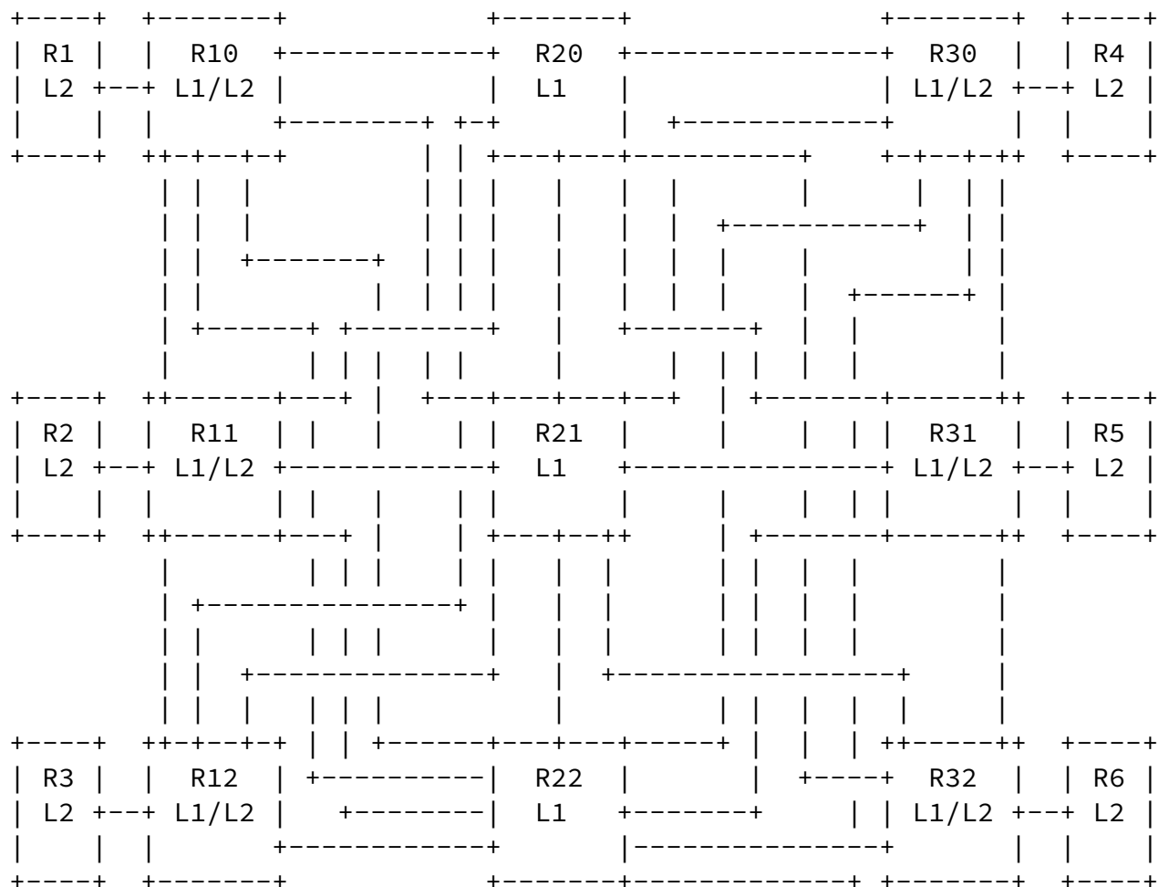
Figure 1: Example topology
