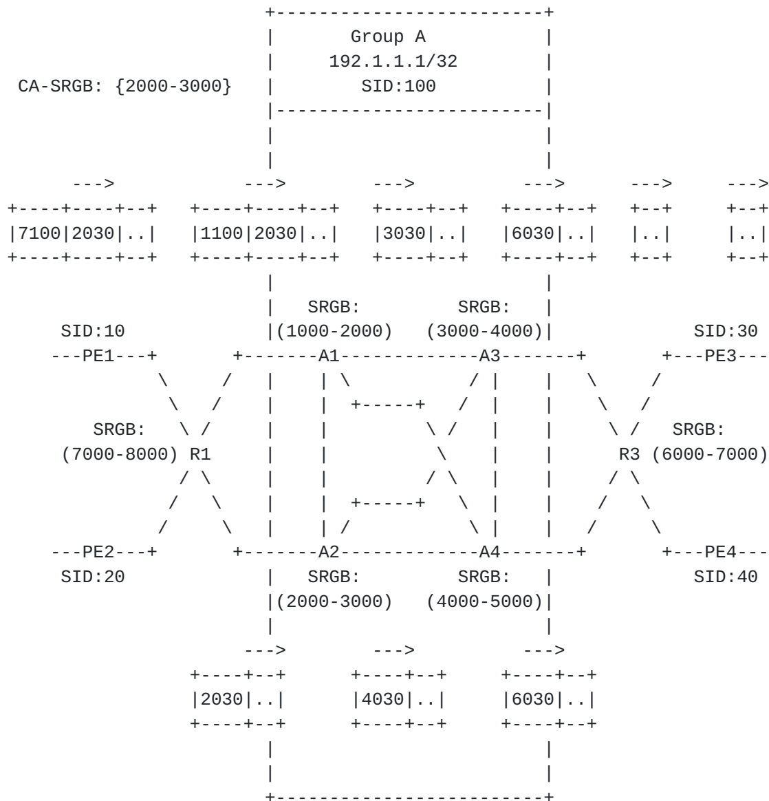
Figure 4: Packet Flow through MPLS-based SR Anycast Segments
