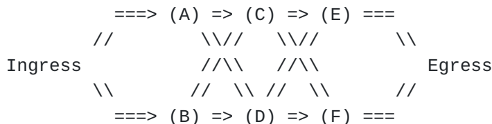
Figure 5: Packet Replication
