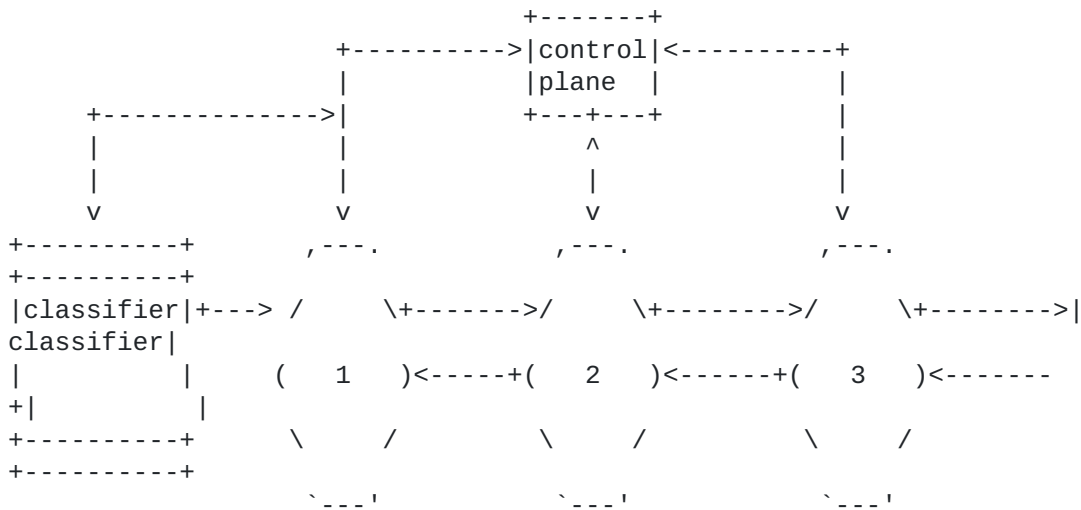
Figure 3: Service Function Chaining Architecture
