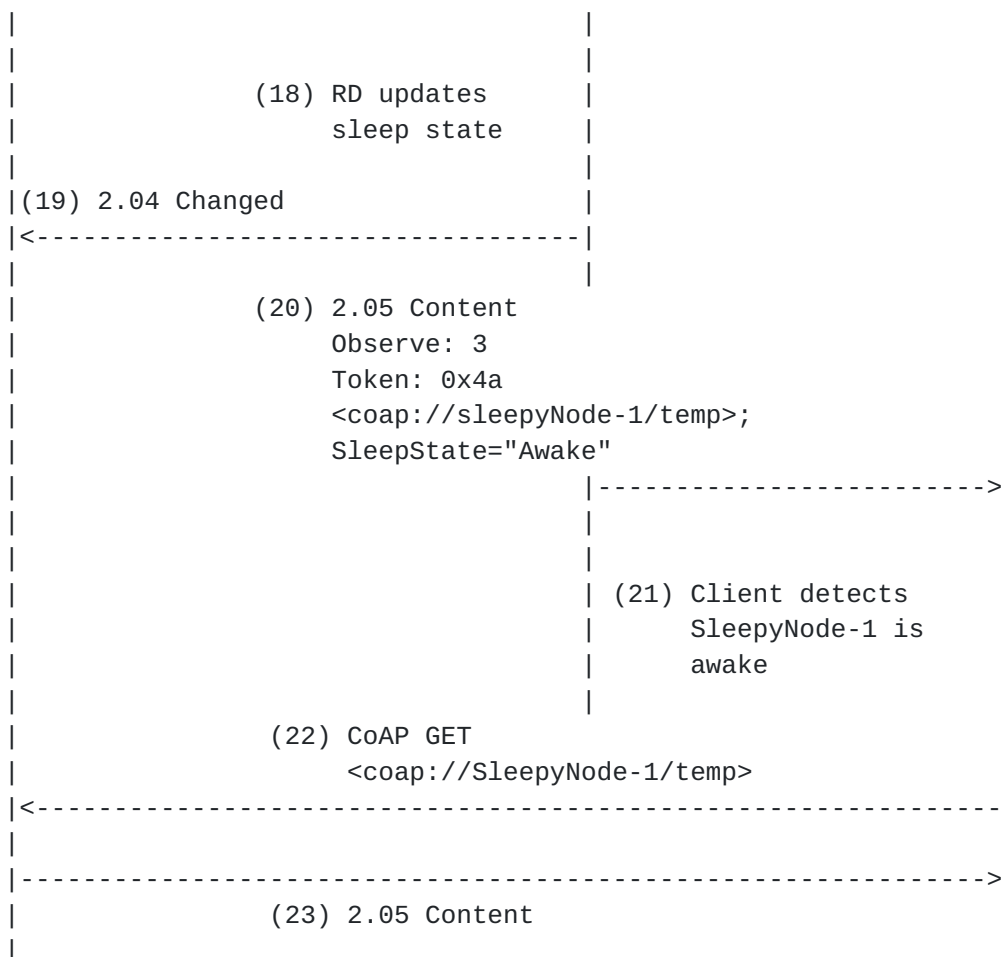
Figure 2: Asynchronous Resource Directory Based Sleep Tracking
