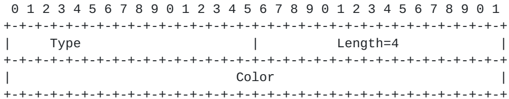
Figure 1: Color TLV
