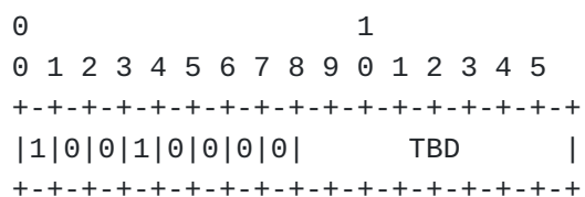
Figure 2: Flags & Type Code Fields
