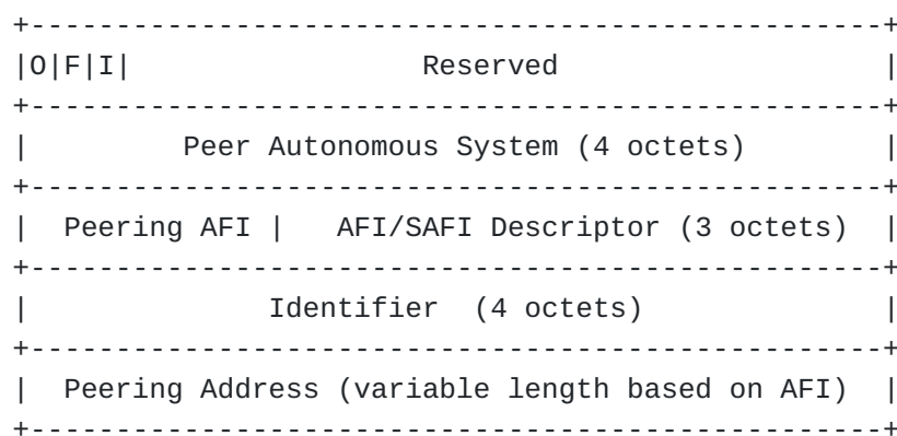
Figure 3: AFI/SAFI Descriptor
