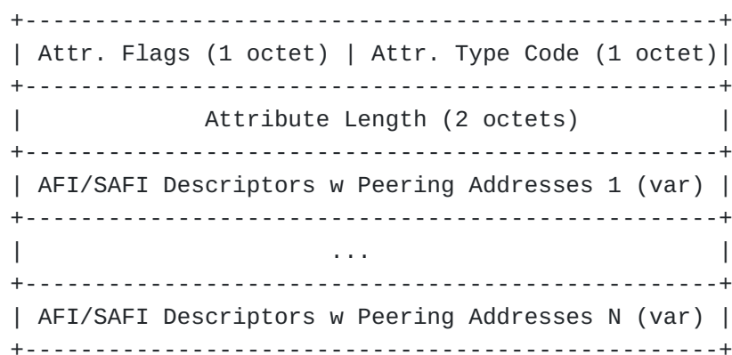
Figure 1: BGP Peer Discovery Attribute
