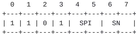
Figure 1: Proposed LOWPAN NHC encoding for AH
