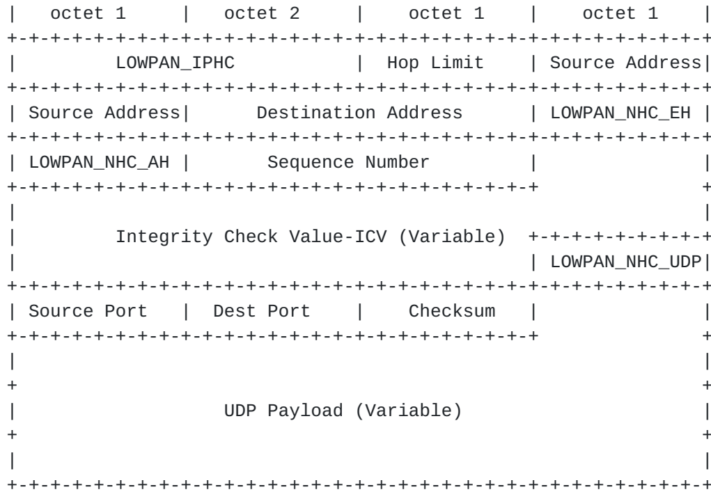
Figure 2: A sample NHC compressed IP/UDP packet secured with AH.
