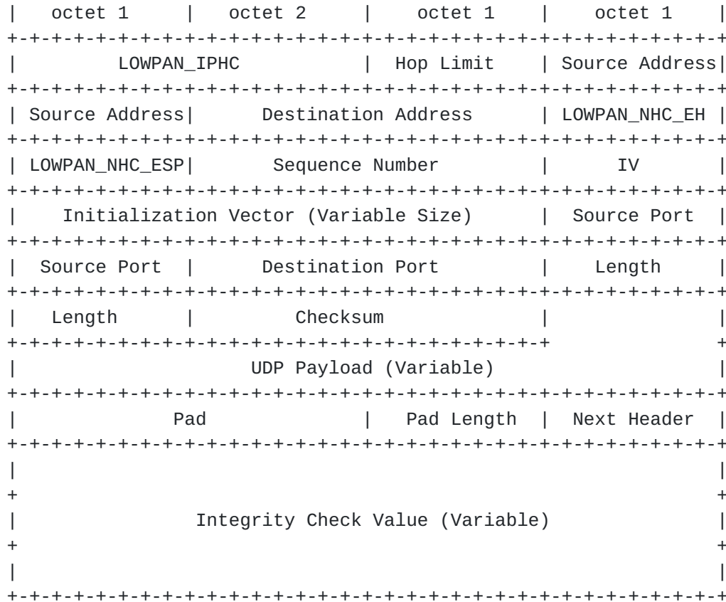
Figure 4: A sample NHC compressed IP/UDP packet secured with ESP.
