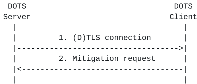
Figure 1: DOTS Signal Channel Call Home Sequence Diagram
