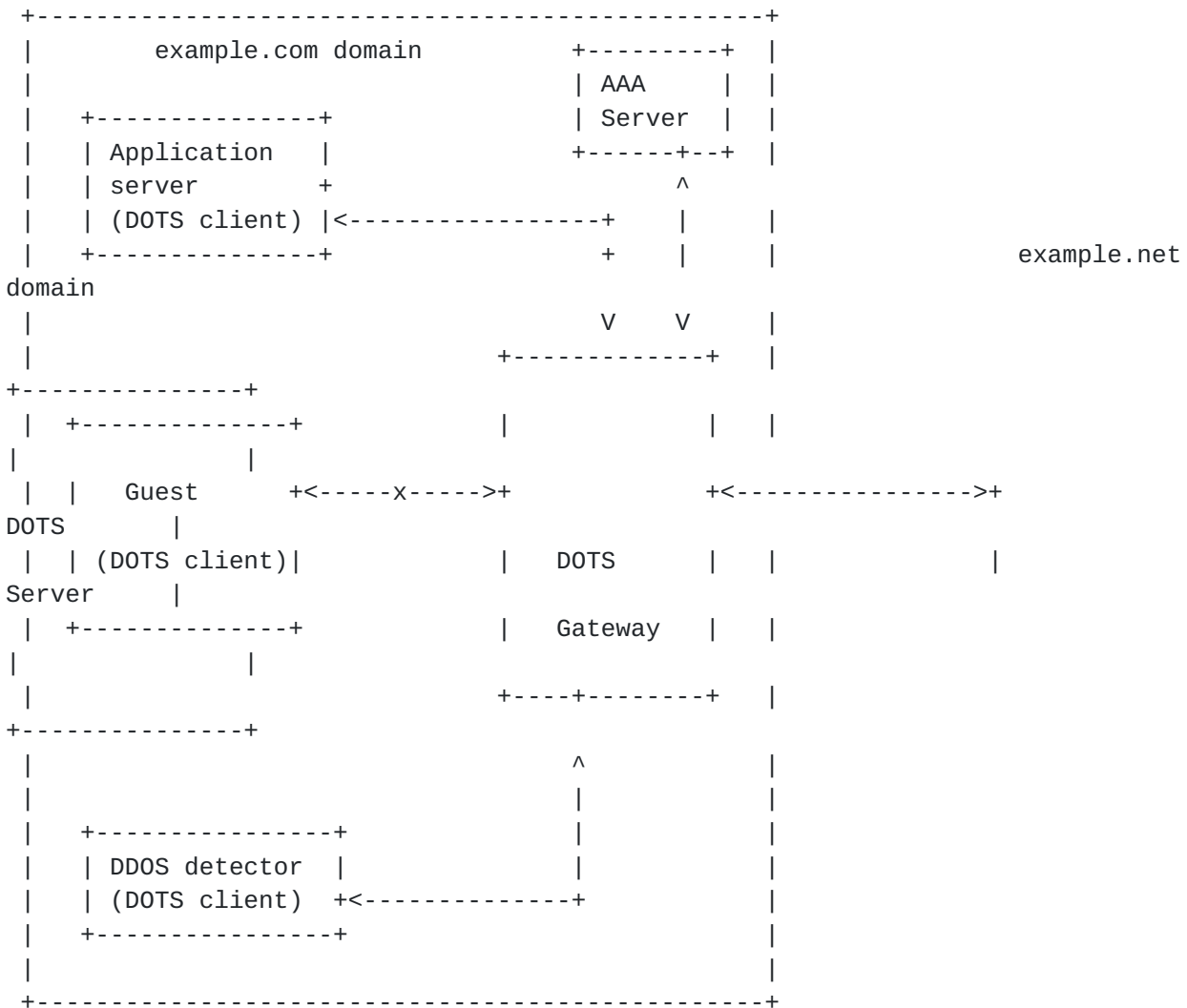
Figure 21: Example of Authentication and Authorization of DOTS Agents
