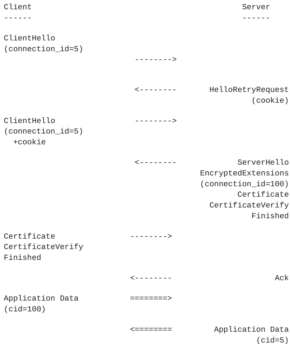
Figure 3: Example DTLS Exchange with Connection IDs
