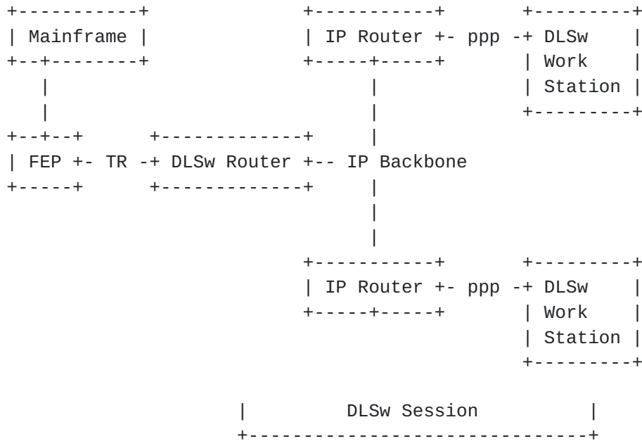
Figure 2-1. Running DLSw on a large number of workstations creates a scalability problem.
