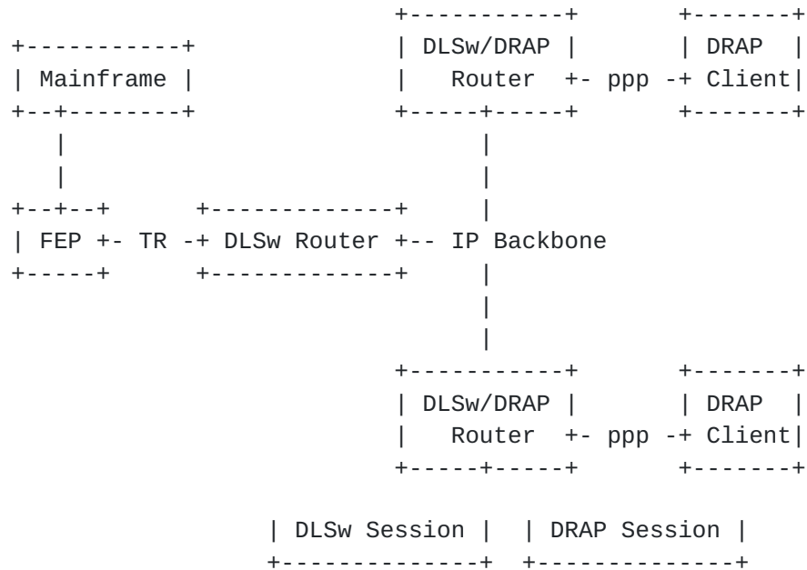
Figure 2-2. DLSw Remote Access Protocol solves the scalability problem.
