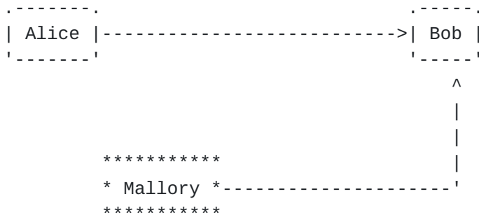
Figure 5: The third kind of attack
