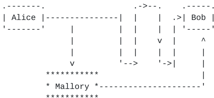
Figure 4: The second kind of attack with bypass
