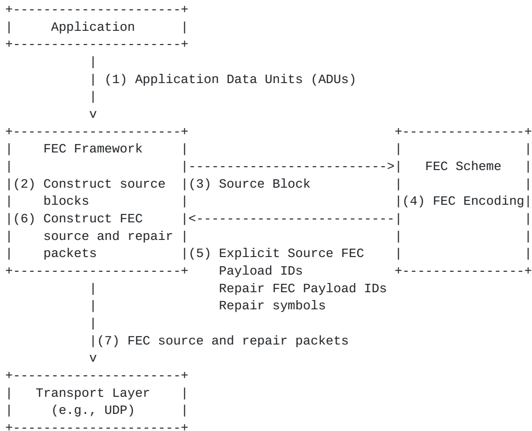
Figure 1: FECFRAME architecture at a sender.
