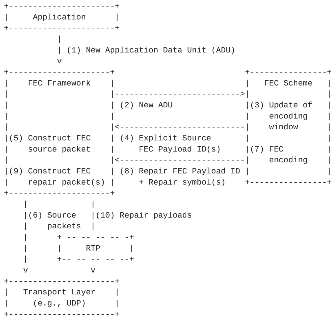
Figure 3: Sender Operation with RTP Repair Flows
