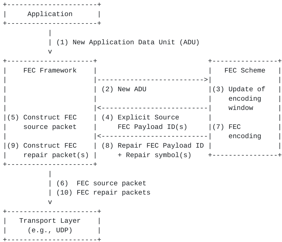
Figure 2: Sender Operation with Convolutional FEC Codes
