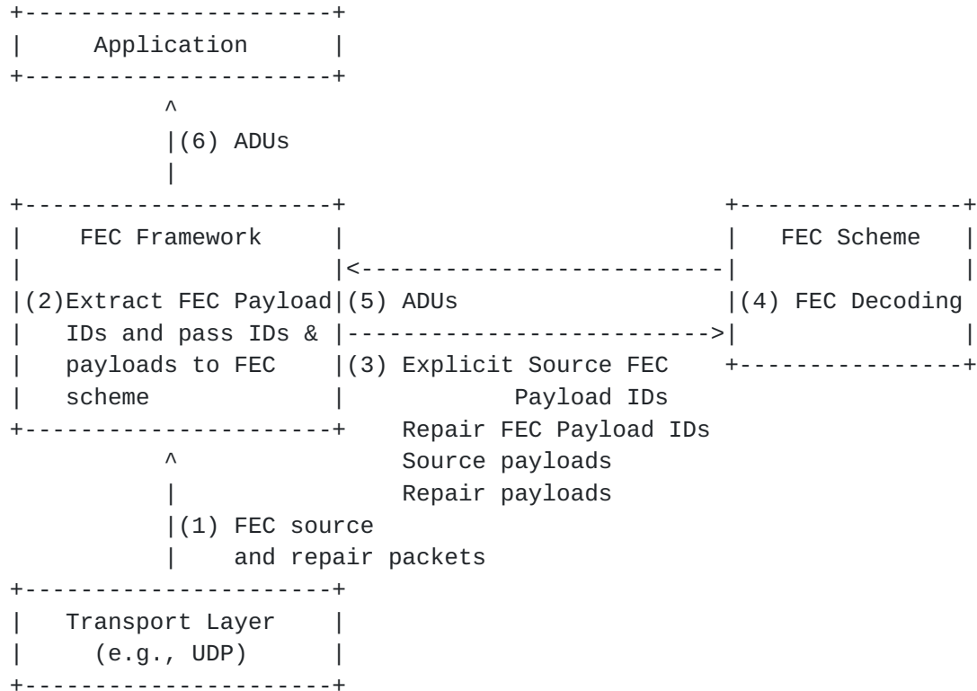
Figure 4: Receiver Operation with Sliding Window FEC Codes
