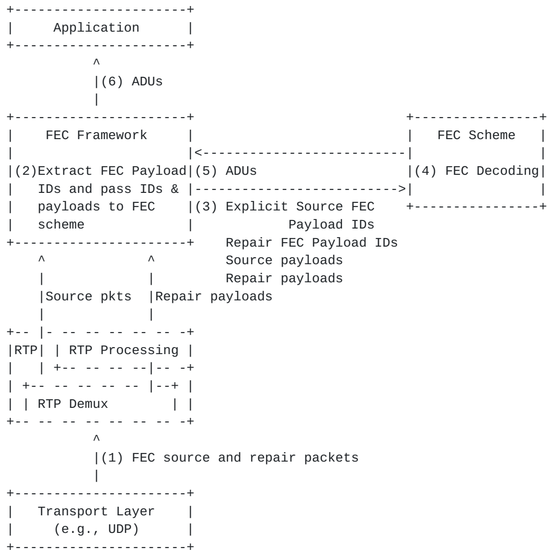
Figure 5: Receiver Operation with RTP Repair Flows
