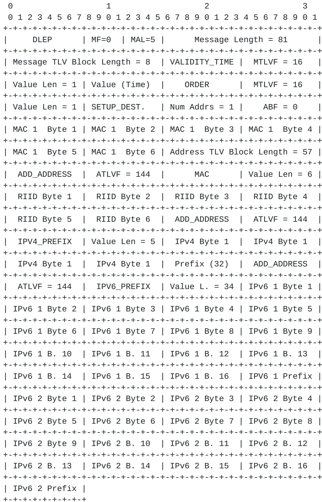
Example of an Setup Destination Order.
