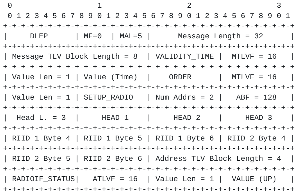
Example of an Setup Router Order.
